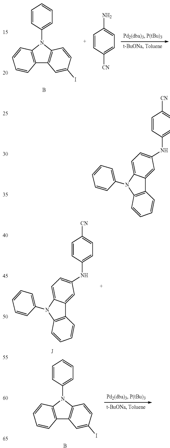
Reaction Scheme 8
