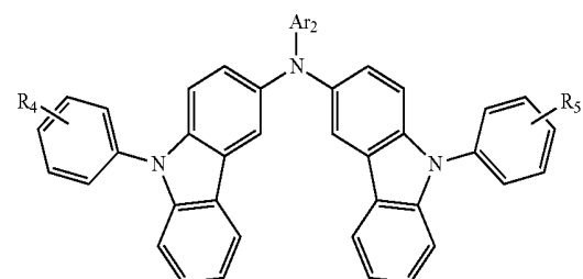
Formula 3
