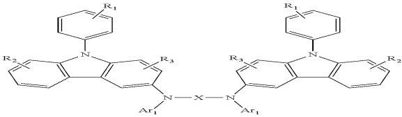
Formula 2
