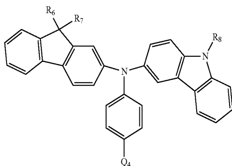
Formula 3a
