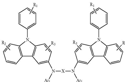
Formula 2
