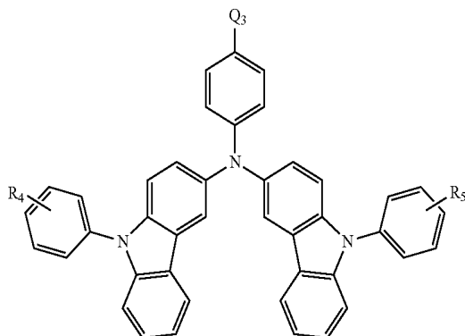
Formula 2a
